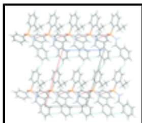
Fig. 2. Packing diagram of the crystal of (I) showing chains of N-H\cdots O intermolecular interactions as viewed down the crystallographic c direction.
